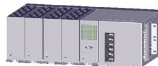
P/N 030-704-20 L0 (Center Mount) Cordex 4kW Shelf Power System with plug in controller & bullet type breaker distribution
